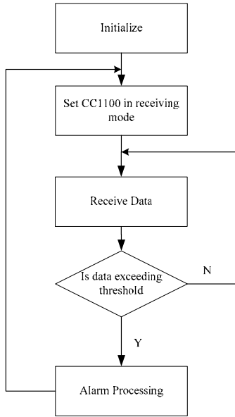
Figure 4. Software flow of center node module
