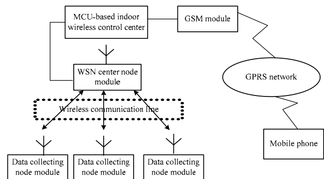
Figure 1. System structural diagram
