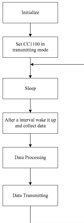
Figure 5. Software flow of data collecting node module
