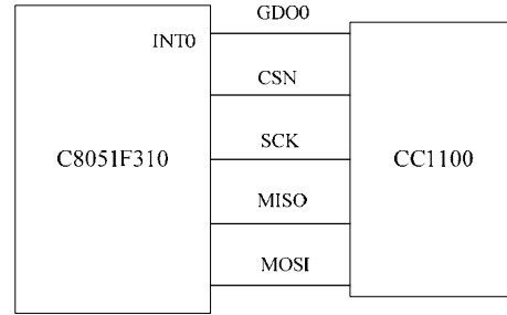
Figure 3. The hardware connection between C8051F310 with CC1100
